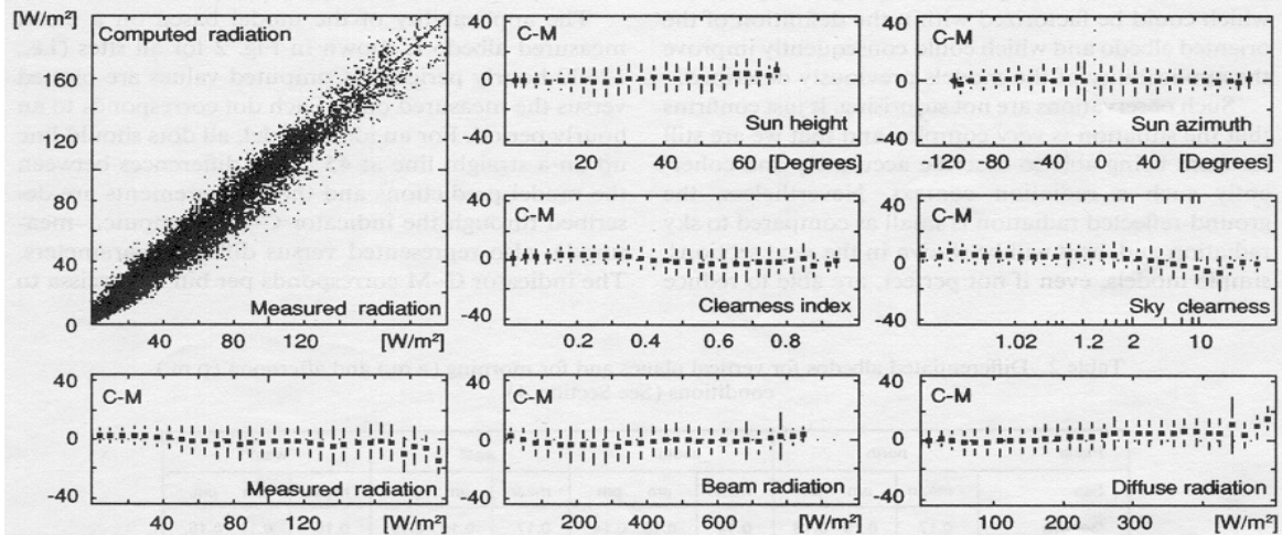
Fig. 2. Applicability of the model for the evaluation of the ground-reflected radiation on a reverse plane with the assumption of an albedo constant and site-dependent. Data include 12600 hourly periods for all sites. The indicator C-M illustrates comparisons between computed and measured values. (See Section 5.)
