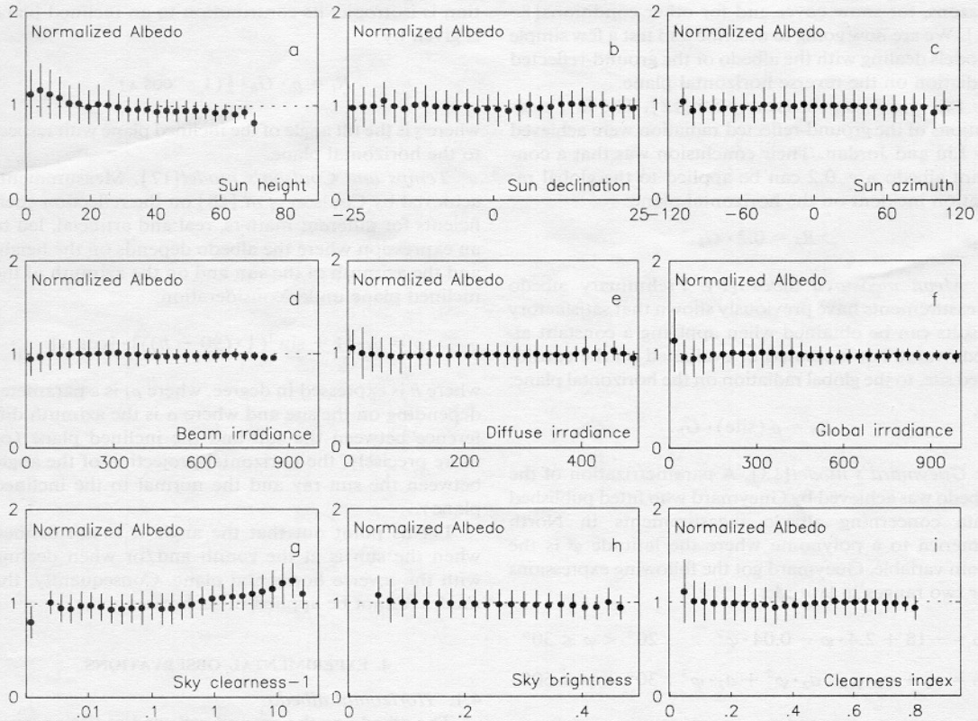
Fig. 1. Albedo variation with data from all sites under consideration. Variations of the albedo with the sun height (a) and with the sky clearness (g) are factorized and extracted for the other graphs (b, c, d, e, f, h, i). (See Section 4.)
